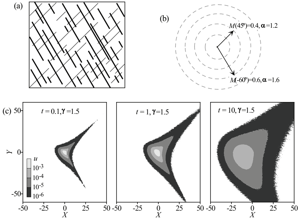
FIGURE 3. Case 1: Conceptual model of a 2- d fracture network (a), the corresponding model parameters (b), and particle tracking solutions (c) to the model equation (9) with \gamma = 1.5 , a = 0.5 , and \mathcal{D} = 1 at time 0.1, 1, and 10, respectively. Initial source location is (0, 0).
