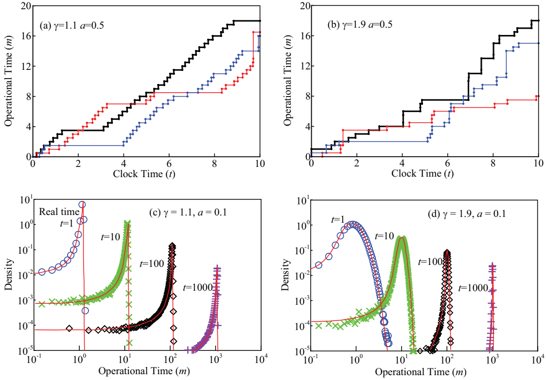
FIGURE 1. Graphs (a) and (b) show three sample paths of the operational time process m = E(t) . For illustration purpose, a large operational time step dm is used. Graphs (c) and (d) show the density h(m, t) of operational time computed via particle tracking (circles) and inverse Fourier transforms (lines).
