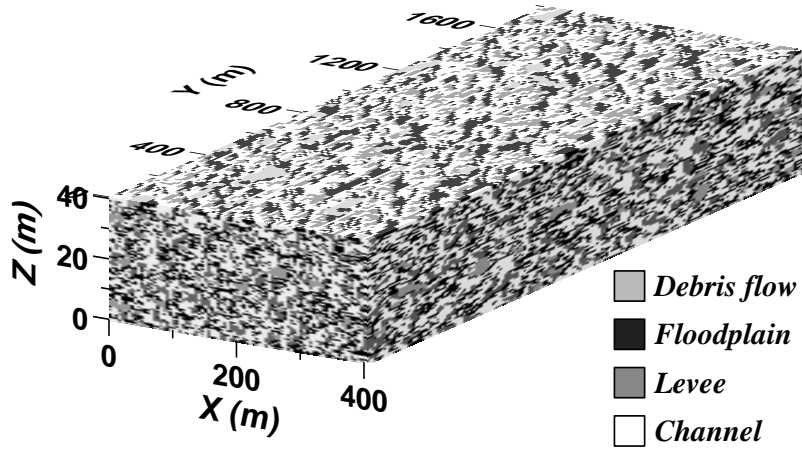
FIGURE 4. Three-dimensional view of synthetic hydrofacies model. For visualization purpose, a different scale is used for each axis.
