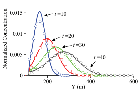
FIGURE 5. Case 2: Plume concentration snapshots at t = 10, 20, 30, and 40 yr respectively, in the direction of flow. Detailed Monte Carlo numerical simulations (symbols) of the 2nd-order advection-dispersion equation versus the best-fit Lagrangian approximations (lines) via the FDE (11) with \gamma > 1 . The FDE is an upscaling model for the more complex Monte Carlo plumes. See the text for model parameters.
