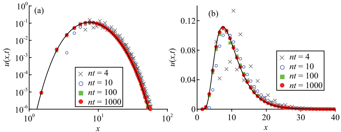
FIGURE 2. Particle tracking solution (circles) versus IFT solution (lines) for the FDE (4) with L = -\partial/\partial x and \gamma = 2 at t = 10 . Graph (b) is the linear-linear plot of (a). The variable nt is the total number of time steps.
