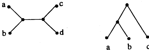
FIG. 2. The quartet ab|cd and the rooted triple ab|c .
