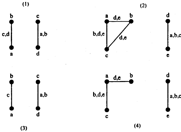
FIG. 7. If R is closed and [R, S] has two components, the either both components have two vertices (1), or one component has three or more vertices (2). In (3) we have removed the triple ab|d from R giving a set that is not closed. In (4) we have removed both bc|d and bc|e , giving a subset of R that is not closed.
