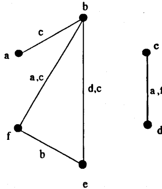
FIG. 4. The graph [R, S] for R = \{ab|c, be|d, be|c, af|g, fe|b, bf|a, bf|c, cd|a, cd|f, cg|b\} and S = \{a, b, c, d, e, f\} . The triples in R with a leaf g are ignored when constructing the graph because g \notin S .
