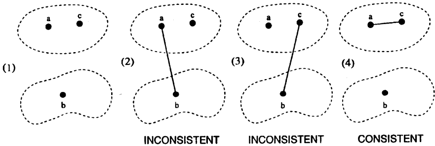
FIG. 6. The components of [R, S] . The dotted lines indicate the components of [R, S] (1). If we add an edge between a and b , (2), or between c and b , (3), then we get a connected graph. Hence, the only triple with these leaves that is consistent with R is ac|b (4).
