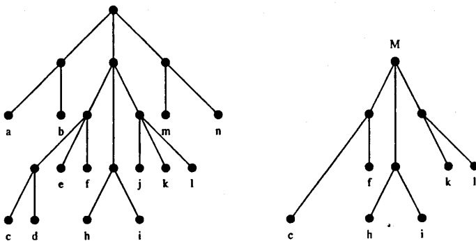
FIG. 5. Given the rooted tree on the left take S = \{c, f, h, i, k, l\} . The induced subtree on the right has the corresponding partition \{\{c, f\}, \{h, i\}, \{k, l\}\} .
