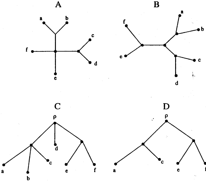
FIG. 1. Four examples of phylogenetic trees . A and B are unrooted . C and D are rooted . B and D are binary .
