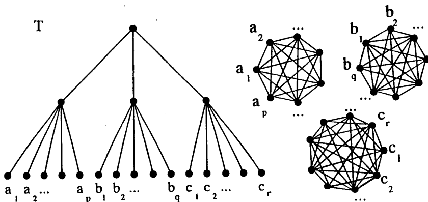
FIG. 8. The tree T on the left is compatible with the set R from Proposition 12, so that R is consistent. On the right is the graph [r(T), \mathcal{L}(T)] , consisting of three disjoint cliques on p , q , and r vertices, respectively. Note that [R, S] is a subgraph of [r(T), \mathcal{L}(T)] for any S (Proposition 8).
