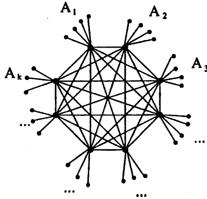
FIG. 3. The graph G with the same quartet set as A_1|A_2|\dots|A_k .
