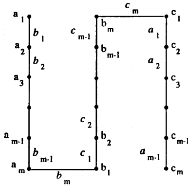
FIG. 10. The graph [R_3, \mathcal{L}(R_3)] . The edges are labelled in italics. The graph is connected, so R_3 is inconsistent by Theorem 2.
