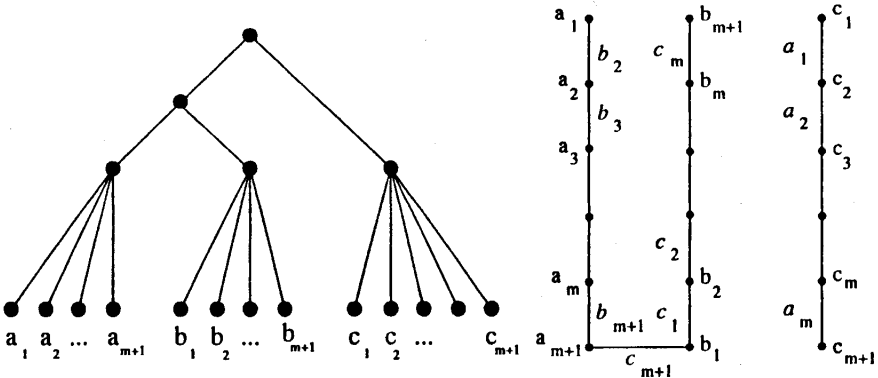
FIG. 9. The tree on the left is compatible with R , so that R is consistent. On the right is the graph [R, \mathcal{L}(R)] and the associated edge labelling.
